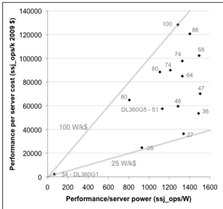
Figure C. 3: Performance Per Watt and Performance per Kilotollar (from Koomey 2009).
