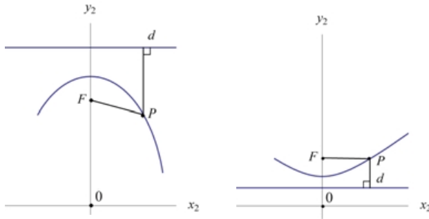
Figure 1 Horizontal cross sections of M' for \varepsilon = 1/2 and \varepsilon = 4
